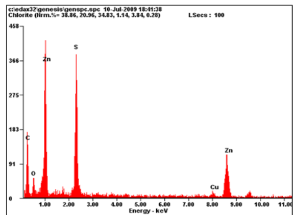
Fig.9: EDAX spectra for ZnS sample
