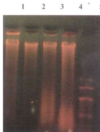
Fig. 2. Metagenomic DNA Lanes 1- uninfected carrot; 2 - carrot infected with Salmonella ; 3 - uninfected cucumber; 4 - cucumber infected with Aeromonas ; 5 - 1 kb DNA ladder
