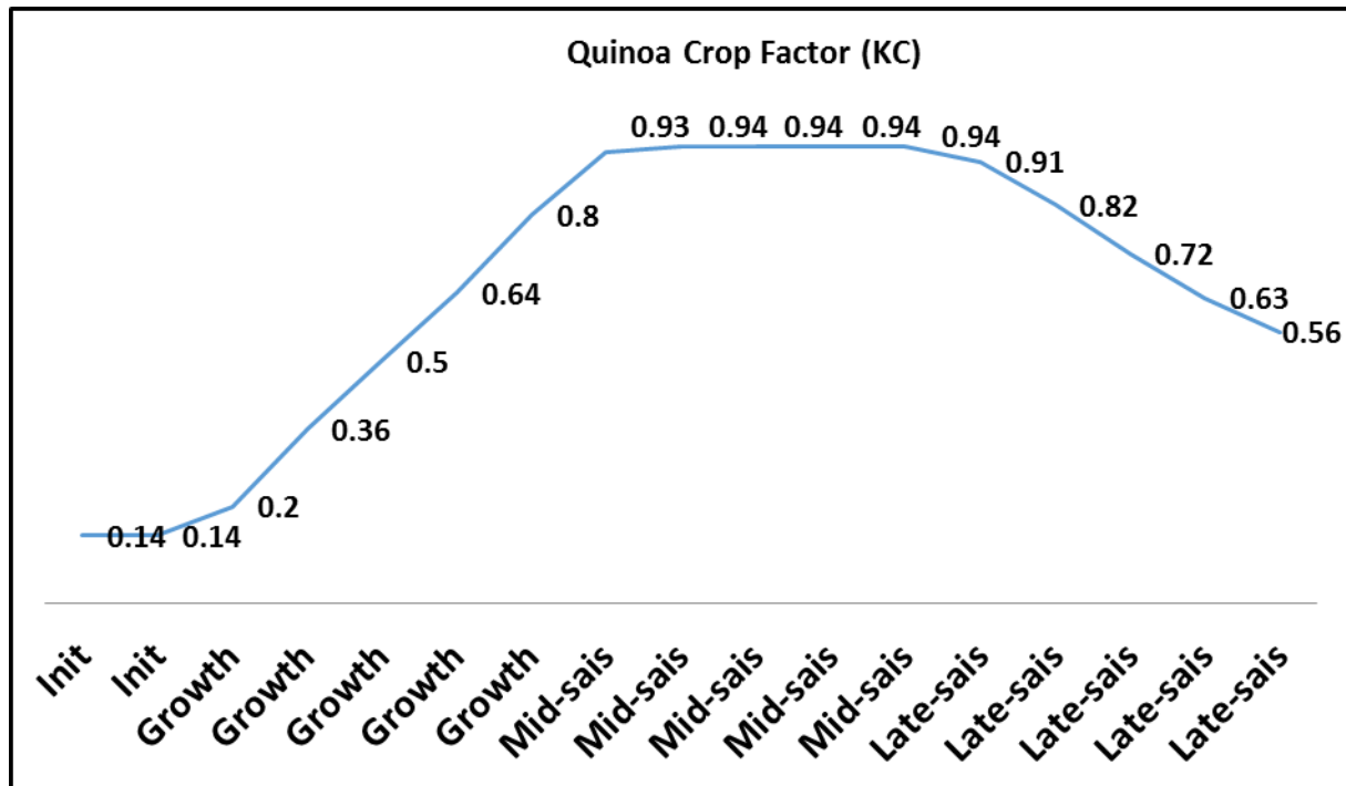
Fig. 4. Variation of quinoa crop factor during the growing period from January to June.
