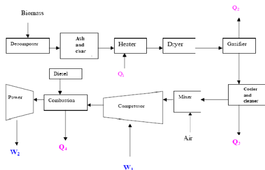
Figure 7. Advanced biomass power with diesel engine (Omer, 2006)
