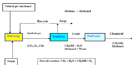
Figure 2. Schematic diagram shows methanol production (Omer, 2006)
