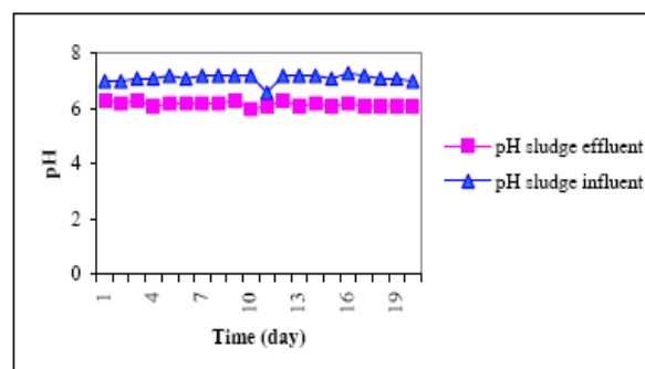
Figure 6. Potential of hydrogen sludge before and after treatment in the digester (Omer, 2006)
