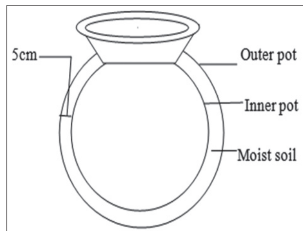
Figure 1: Double wall pot
