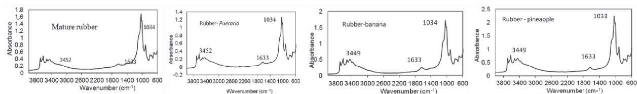
Fig. 1. FTIR spectra of different rubber based systems at Amayannoor
