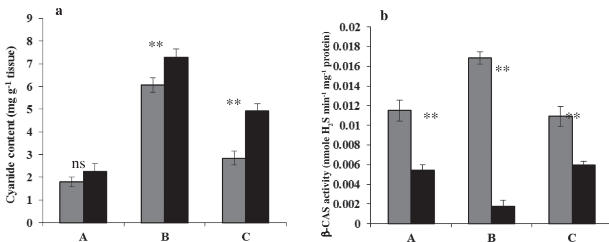
Fig. 4. a) Cyanide content and b) \beta -CAS activity in the bark tissues of healthy (■) and stress exposed (■) Hevea brasiliensis . A) Root stock; B) Tapping panel; C) Above tapping panel [Values \pm SE, ns=not significant; ** P \leq 0.001 ]
